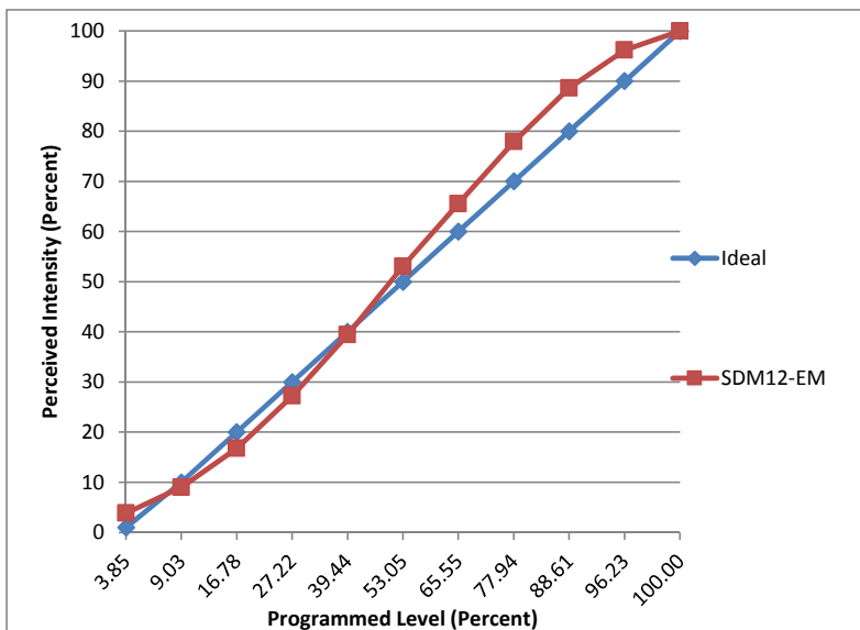
Linearity Curves (Best-fit Power Profile Applied):
